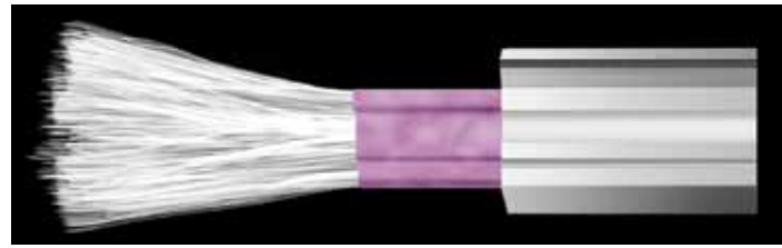
Strands of reinforced glass fibers are soaked in resins, then pulled through heated dies to create FiberCore™, which is married to an exterior PVC surface, and fusion welded at the window corners.
